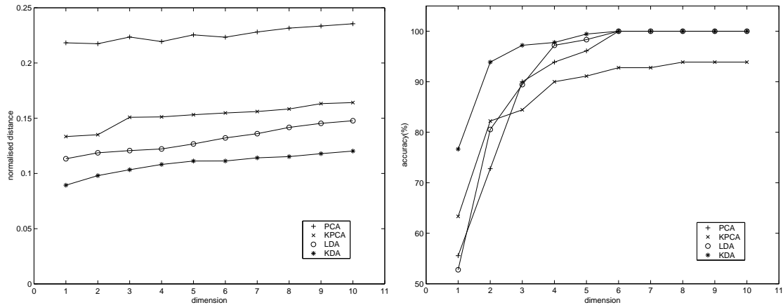
(a) Recognition robustness
