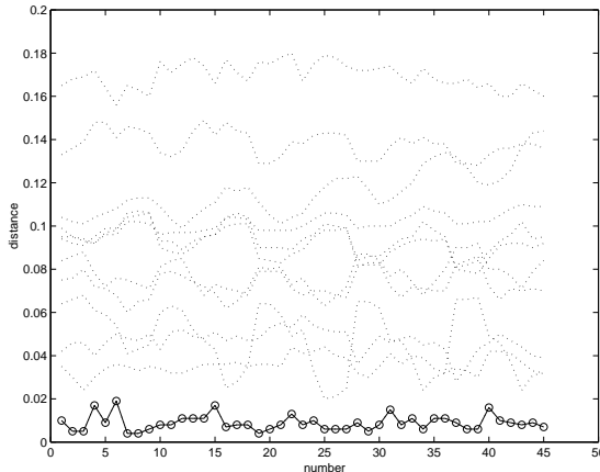
Figure 6: Recognising multi-view faces using distances to the identity surfaces . The solid line denotes the results of the ground-truth subject.
