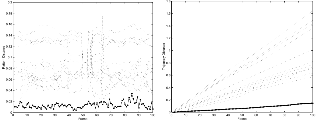
Figure 11: Pattern distances and trajectory distances. The ground-truth subject is highlighted with solid lines. By using KDA and identity surfaces , the pattern distances give good recognition for individual frames. However, the trajectory distances provide a more robust performance, especially its accumulated effects (i.e. discriminating ability) over time.
