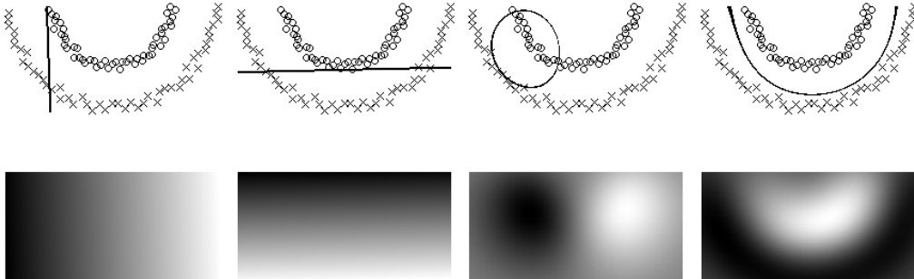
Figure 1: Solving a nonlinear classification problem with, from left to right, PCA, LDA, KPCA and KDA.
