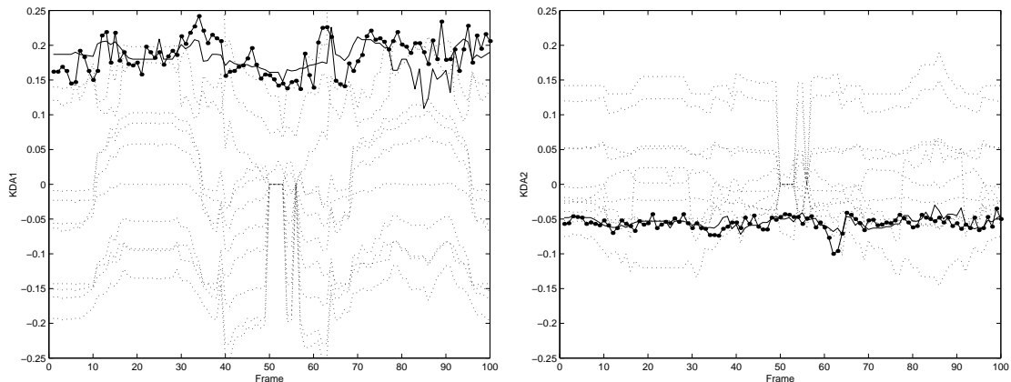
Figure 10: The object and model trajectories in the first two KDA dimensions. The object trajectories are the solid lines with dots denoting the face patterns in each frame. The others are model trajectories where the ones from the ground-truth subject highlighted with solid lines.
