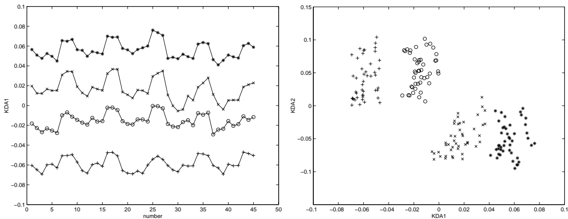
Figure 4: Distribution of the KDA patterns obtained from the same face images as in Figure 3.
