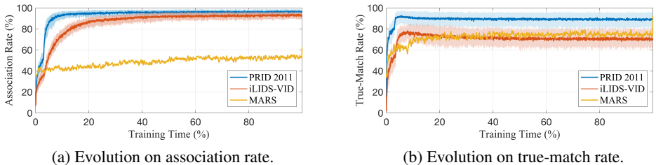
Figure 4: Evolution on cross-camera tracklet association. The shaded areas denote the varying range of 10-split results repeated on PRID 2011 and iLIDS-VID. Best viewed in colour.
