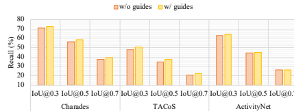
Fig. 6. Effectiveness of guided attention mechanism by comparing with the conventional attention modules [20].
