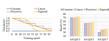
Fig. 5. Effects of constructing elastic boundary subject to an evolving threshold on Charades-STA.
