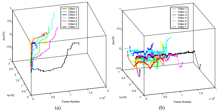
Figure 5: (a) and (b) show the first 2 principal components of \widetilde{\mathbf{sv}}_t over time and colour histogram for seven different aircraft docking videos respectively. Note that PCA is just for visualisation here. Each element of \widetilde{\mathbf{sv}}_t and colour histogram is normalised to have a value range of [0, 1] .
